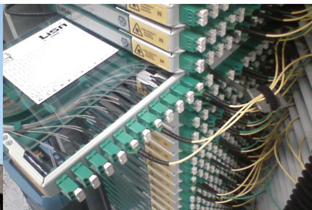
P2P Architecture
